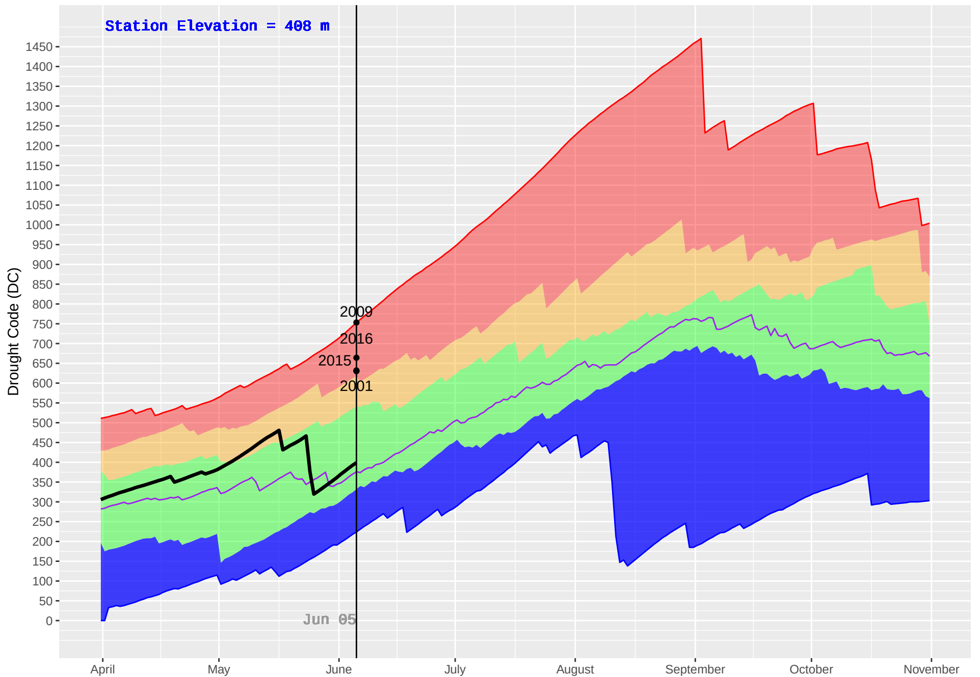
LILLOOET (280) : Historical (1977–2018) and Current (2019) Daily Drought Code (DC)
