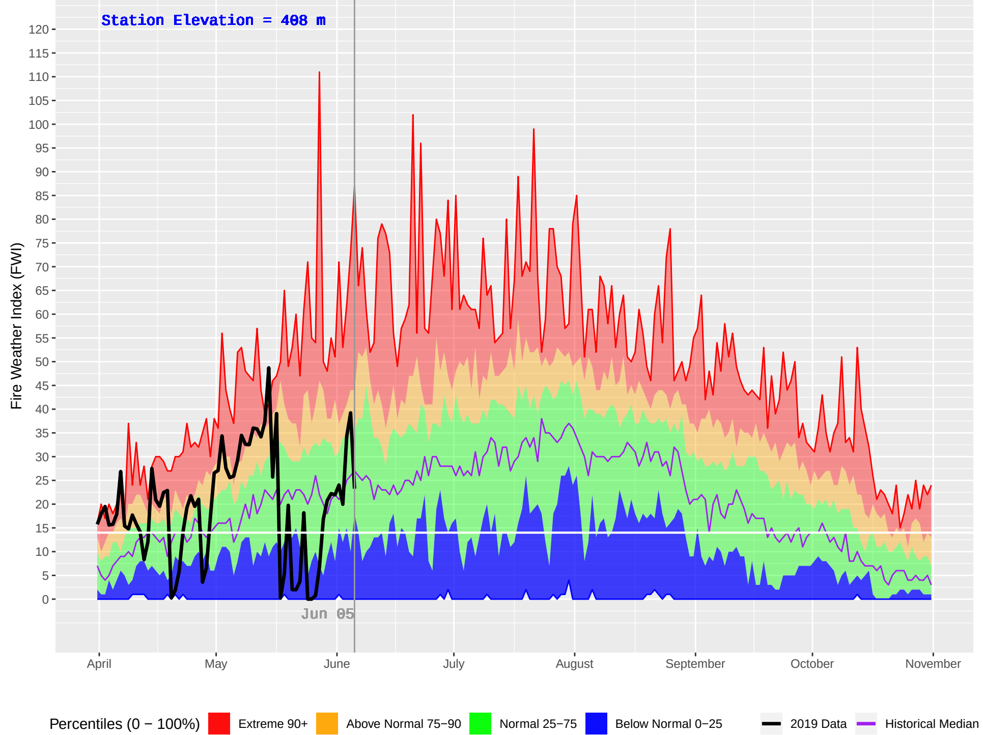
LILLOOET (280) : Historical (1977–2018) and Current (2019) Daily Fire Weather Index (FWI)
