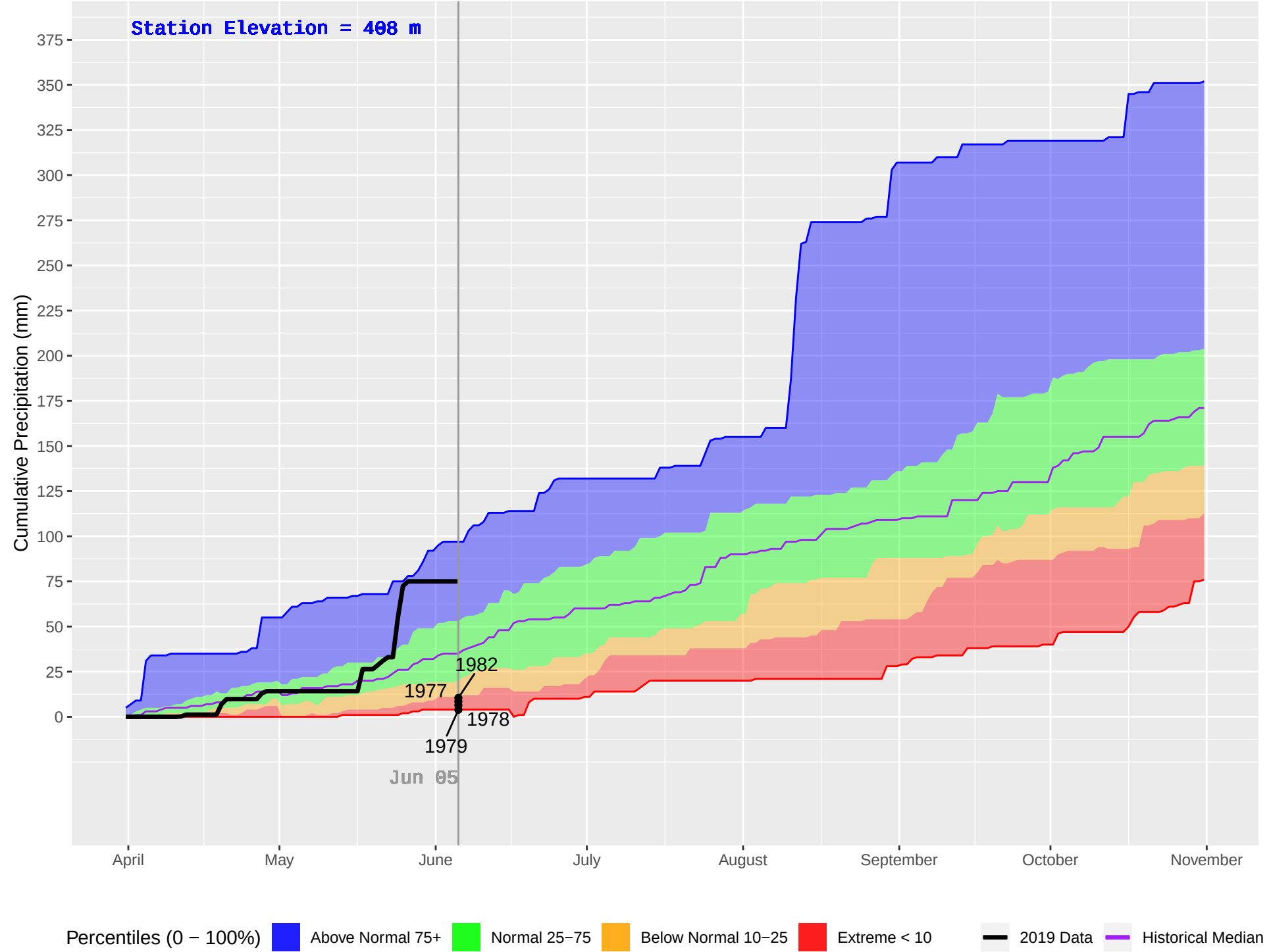
LILLOOET (280) : Historical (1977–2018), Current (2019) Daily Cumulative Precipitation
