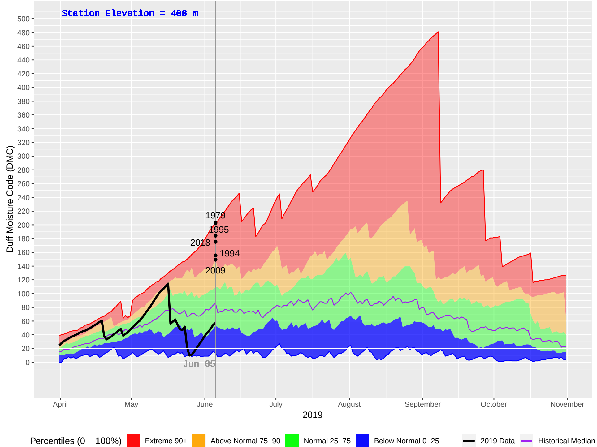
LILLOOET (280) : Historical (1977–2018), Current (2019) Daily Duff Moisture Code (DMC)
