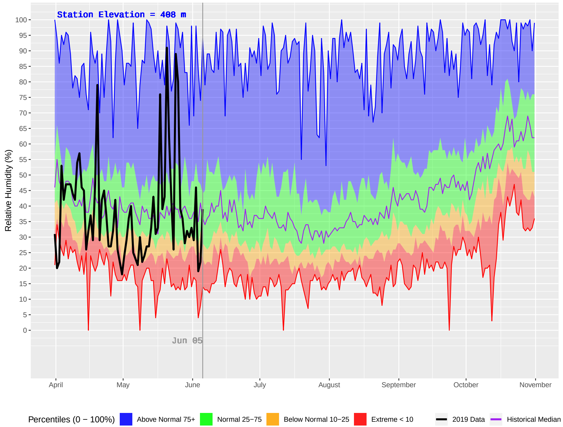
LILLOOET (280) : Historical (1977–2018) and Current (2019) Daily Relative Humidity
