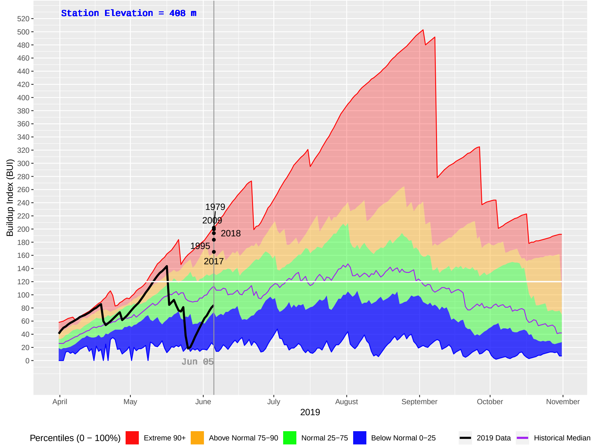
LILLOOET (280) : Historical (1977–2018), Current (2019) Daily Buildup Index (BUI)
