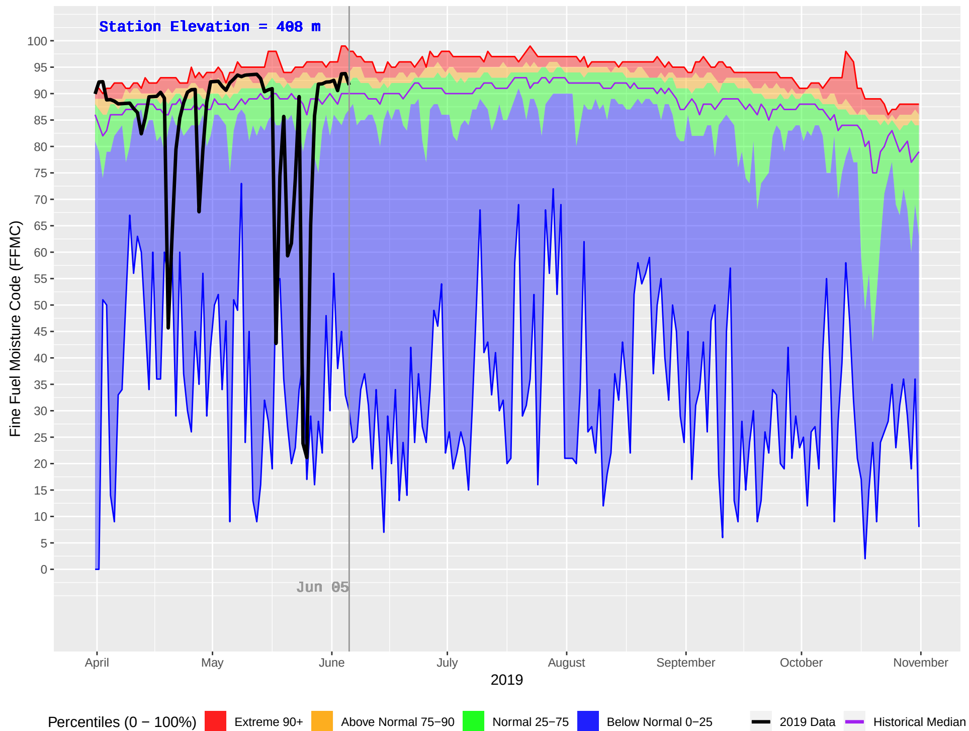
LILLOOET (280) : Historical (1977–2018) and Current (2019) Daily Fine Fuel Moisture Code (FFMC)
